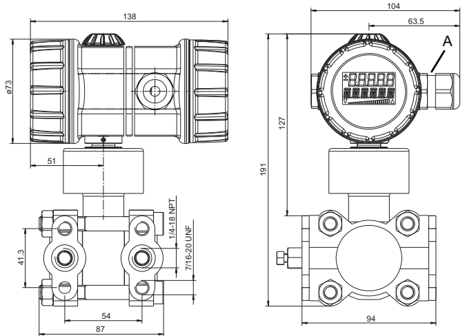
Type 403022/0-0-2 (long, stainless steel, with cable gland)
